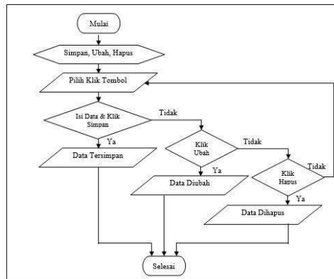
Gambar 3.9 Flowchart Form Sistem
