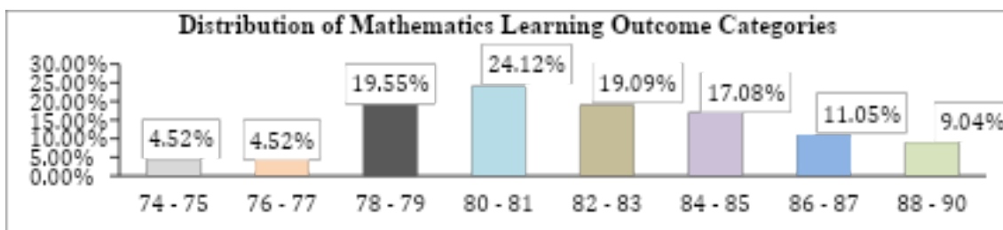
Figure 4. Frequency of Interval Data on Mathematics Learning Outcomes
