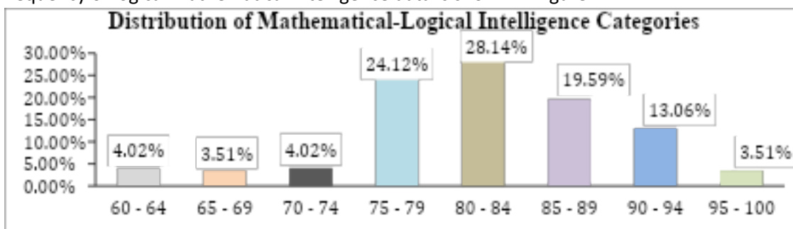
Figure 1. Frequency of Intervals of Mathematical-Logical Intelligence Data
